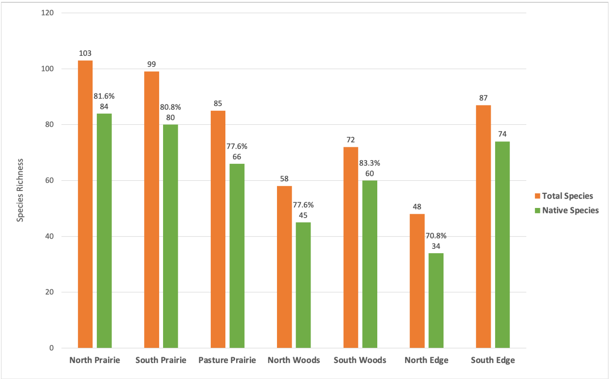
Figure 1. Species richness and native species representation across transects. Bars show total species richness and native species richness for each transect. Percent values indicate the proportion of native species relative to total species richness within each transect. Differences among transects reflect variation in community composition across habitats.
