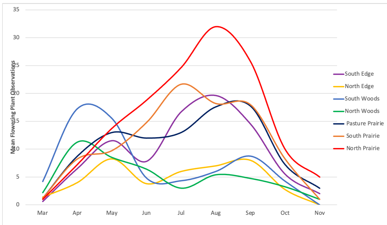
Figure 2. Seasonal patterns in flowering plant observations across habitats during the 2022 phenology season. Lines represent seven monitoring transects through the prairie, woodland and edge-only habitats. Values represent the mean number of flowering plant observations per sampling event within each month. Monthly means were used to account for variation in sampling frequency and allow comparison of seasonal flowering activity among transects.
